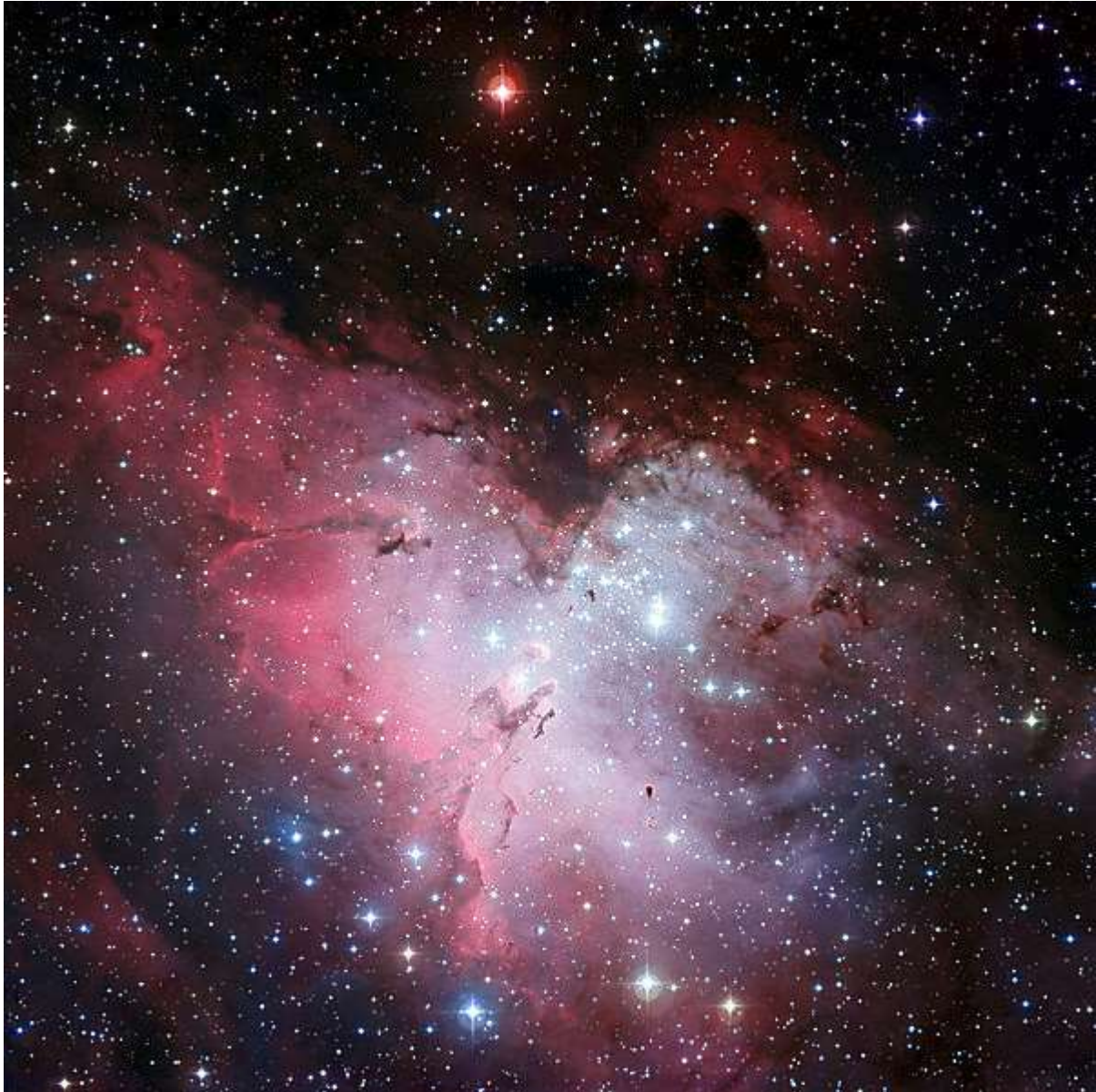
M16 : Nébuleuse de l'Aigle. Images obtained with the Wide-Field Imager camera on the MPG/ESO 2.2-metre telescope at the La Silla Observatory. http://www.eso.org/public/images/eso0926a/
